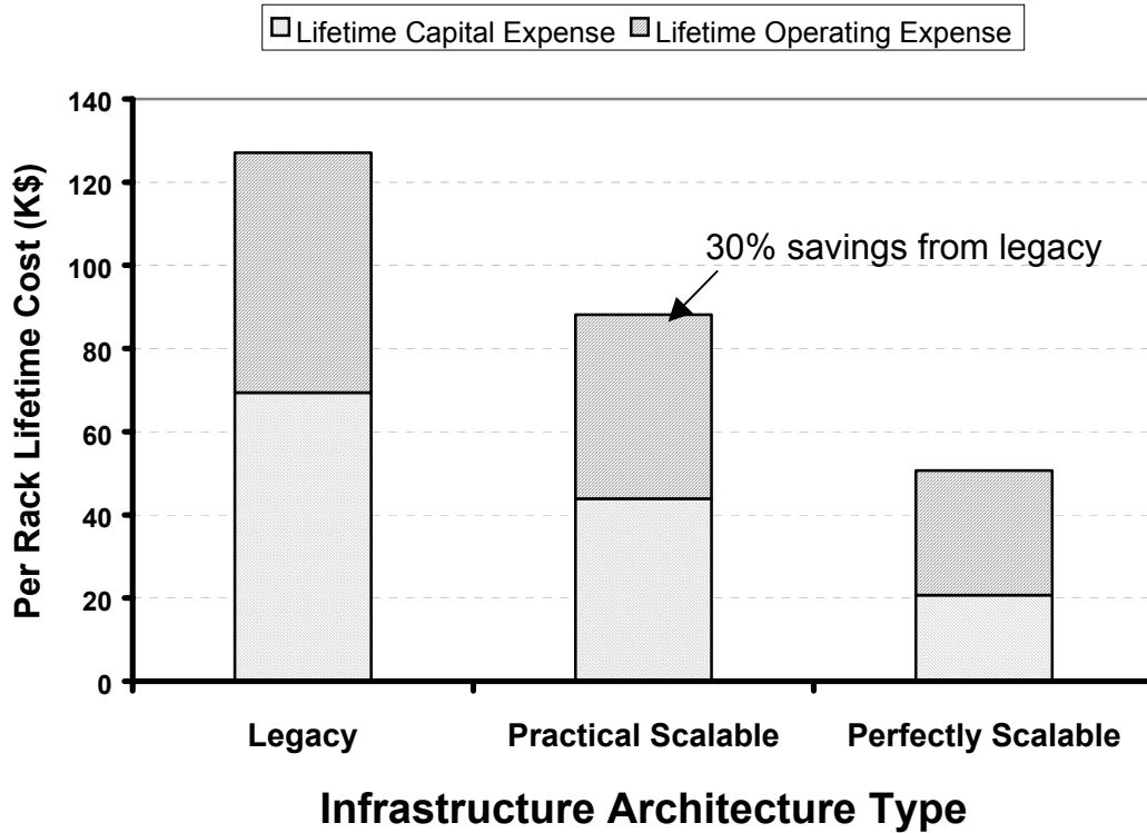
Figure 3 – Per Rack Lifetime Cost for Three Types of Data Center and Network Room Infrastructure Types
