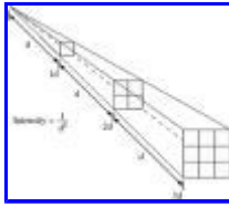
Figure 2-1 Inverse Square Law
